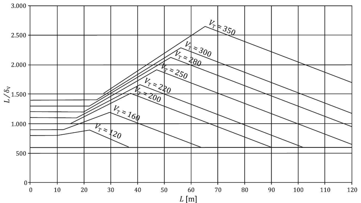
Figure A.2.3 — Maximum permissible vertical deflection \delta_v for railway bridges with 3 or more successive simply supported spans corresponding to a permissible vertical acceleration of b_v = 1 [m/s 2 ] in a coach for speed V_T [km/h]
