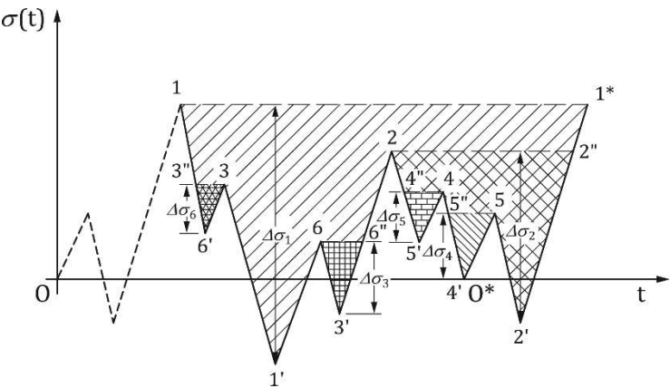
Figure F.6 — Example of reservoir method
